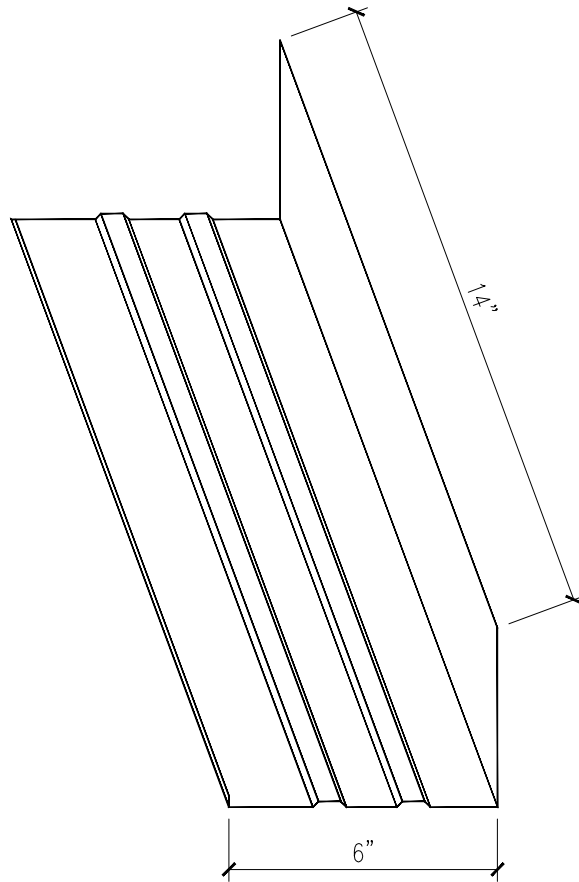
STEP FLASHING
