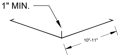
OPT. A - STANDING SEAM VALLEY METAL
