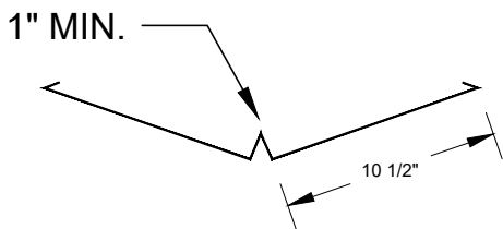
OPT. A - SINGLE DIVERTER VALLEY METAL
